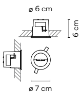
Remote Built-in Canopy E4 Ø 110 mm. Watt-Optionen: >25W. <240W.
